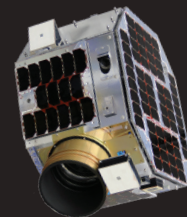
NAUTILUS – up to 150 kg 60 x 60 x 60 cm, scalable Payload: up to 90 kg, 525 W
