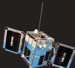
DEFIANT – up to 50 kg 36 x 36 x 45 cm, scalable Payload: up to 30 kg, 215 W
